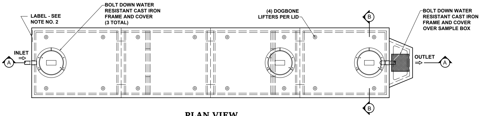
PLAN VIEW
