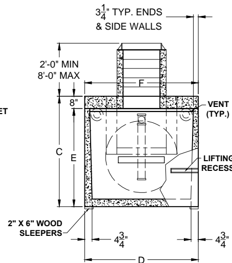
SECTION THRU "B-B"
