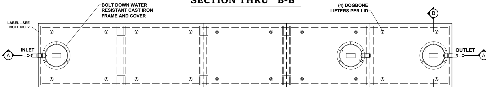
PLAN VIEW
