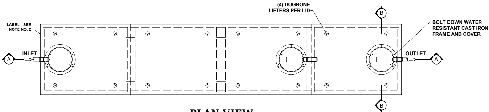
PLAN VIEW
