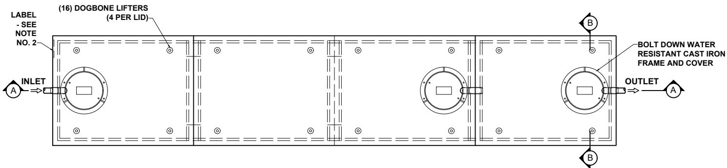
PLAN VIEW
