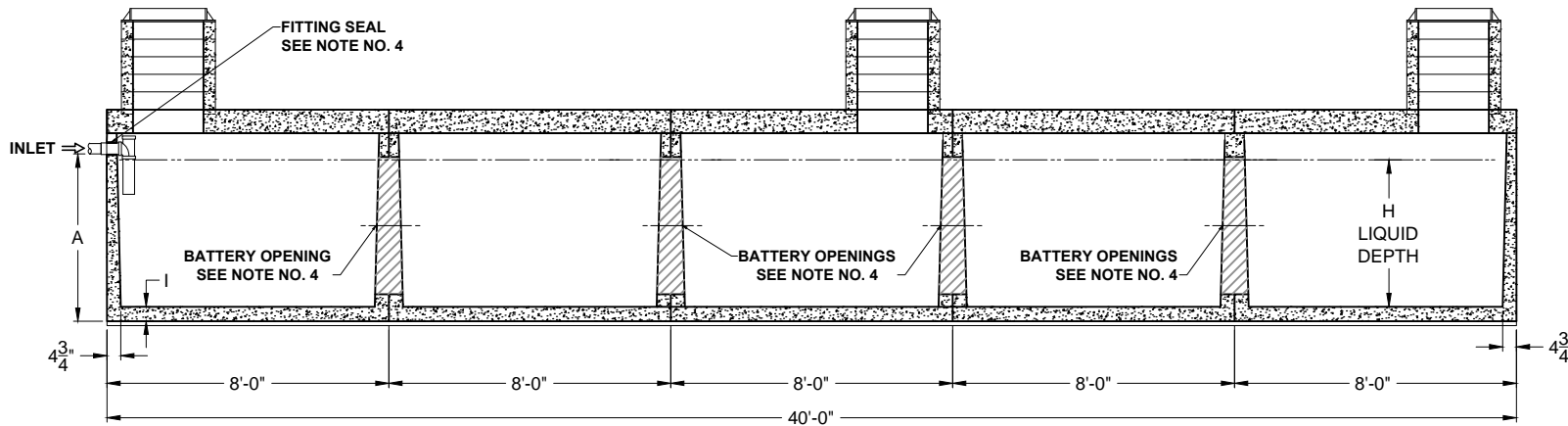
SECTION THRU "A-A"
