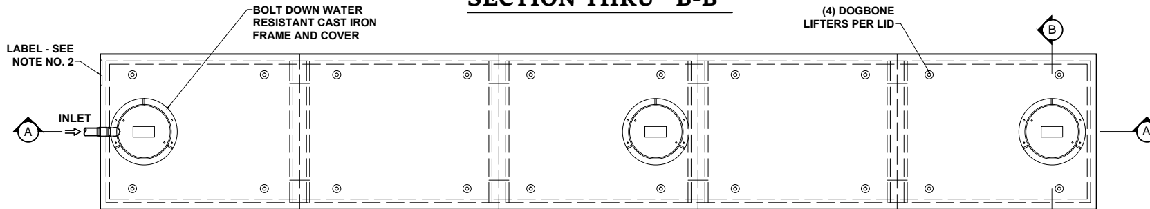
PLAN VIEW
