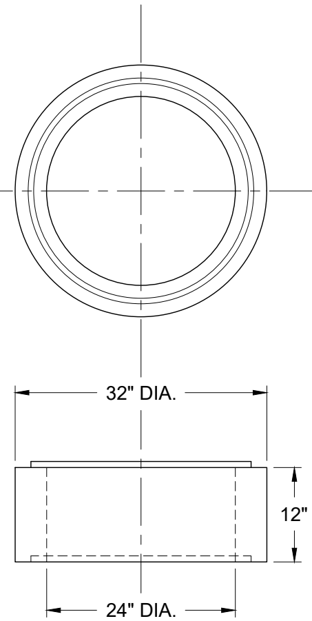
12" GRADE RING
