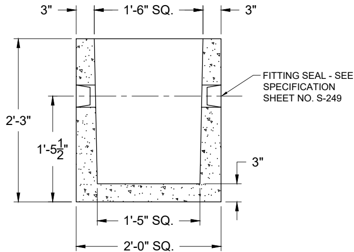
SECTIONAL VIEW
