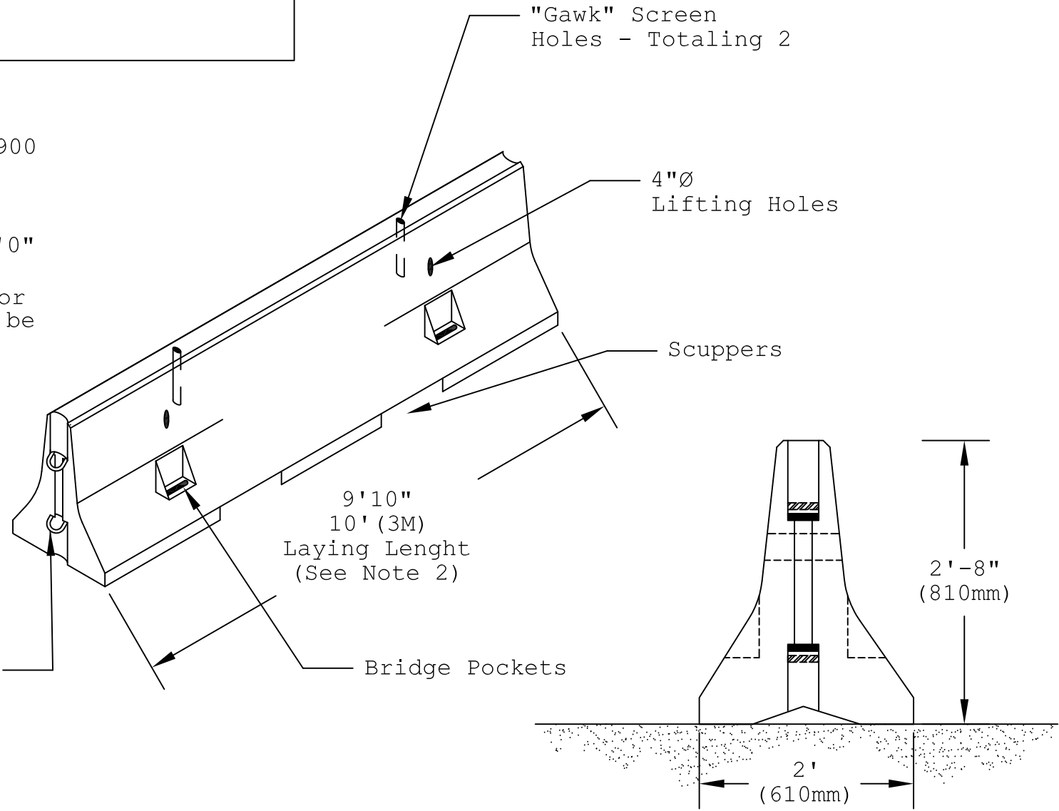
Barrier End Detail
