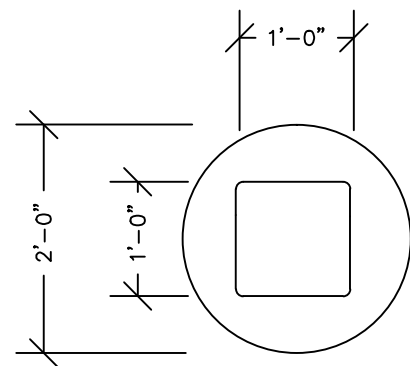
4 PC POST DETAIL (BELOW SUB-GRADE) N.T.S
