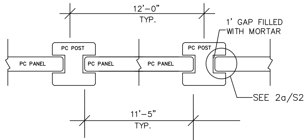
2 PANEL ASSEMBLY PLAN N.T.S
