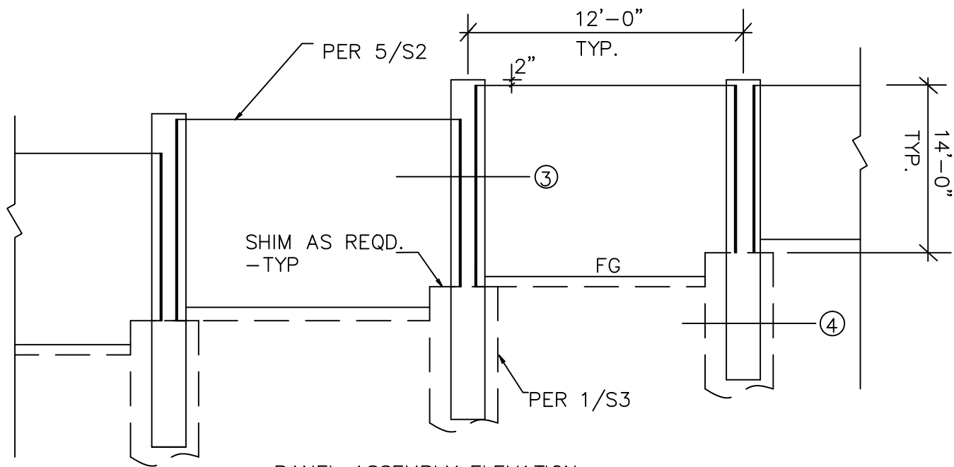
1 PANEL ASSEMBLY ELEVATION N.T.S
