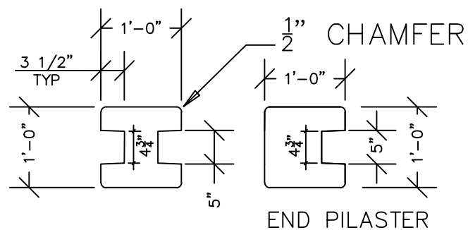
3 PC POST DETAIL (ABOVE SUB-GRADE) N.T.S
