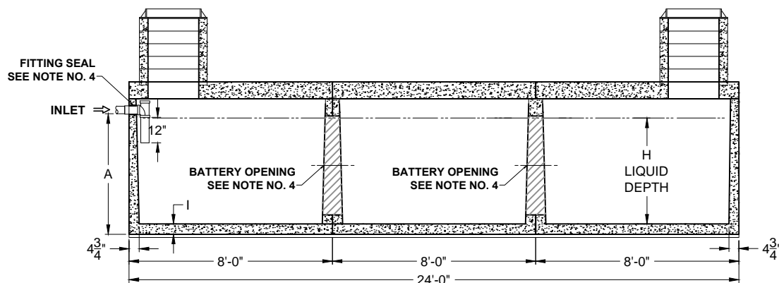
SECTION THRU "A-A"
