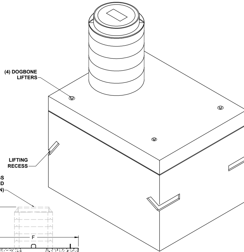
ISOMETRIC VIEW
