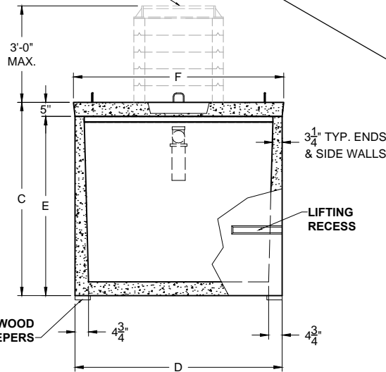
SECTION THRU "B-B"
