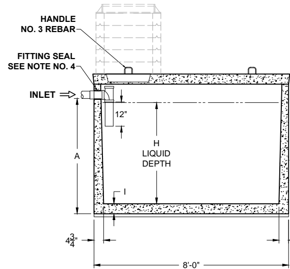
SECTION THRU "A-A"
