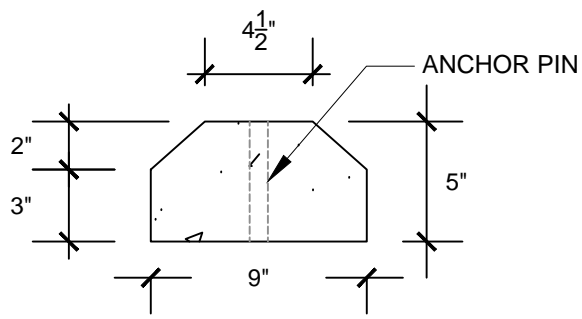
END DETAIL
